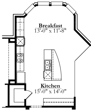
Optional Kitchen Layout
