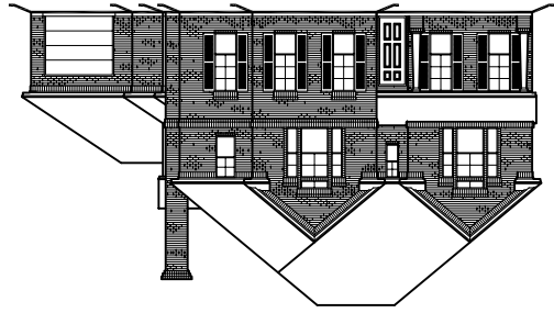
Elevation "E"
